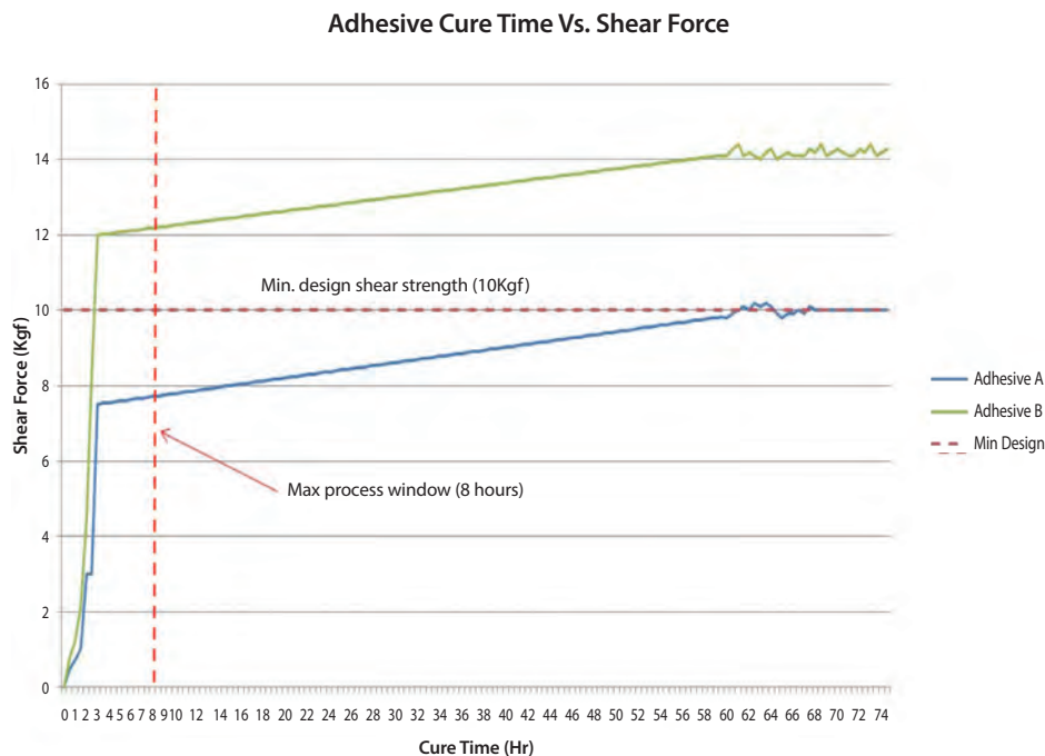
Figure 1. Adhesive die shear results.
