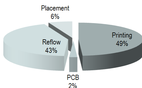
Fig6. Repartition of the 01005 defects root causes
