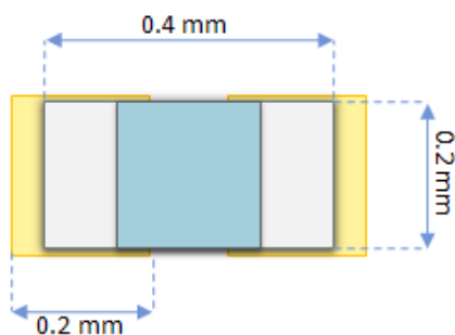
Fig3. 01005 and pad dimensions
