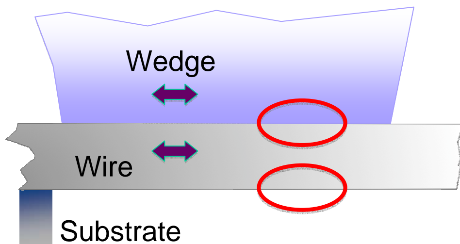
Fig. 1 First or cleaning phase of wedge bonding
