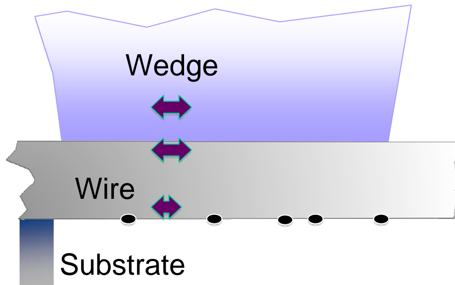
Fig. 2 Second or incipient bonding phase of wedge bonding
