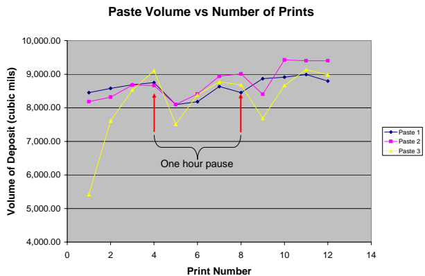
Figure 8. Printed volume versus print number in the 12 board paste evaluator. Note that we could eliminate Paste 3 after just this test as it has an unacceptable response to pause and poor printed volume consistency.
